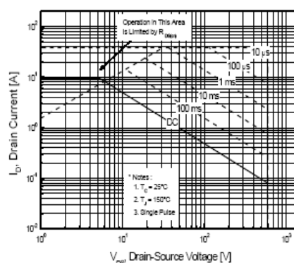
Figure 9-2. Maximum Safe Operating Area for HM10N65F
